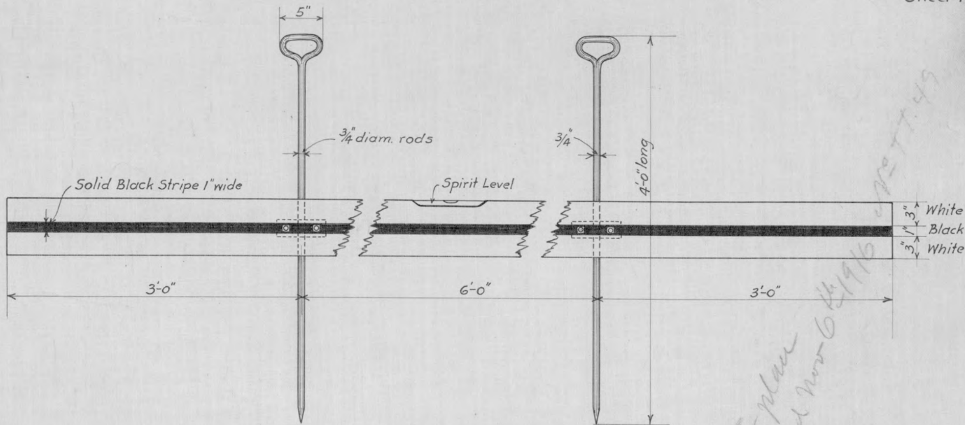
Front Elevation.
