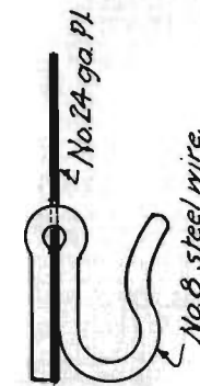
LAMP HOOK. Full Size.
