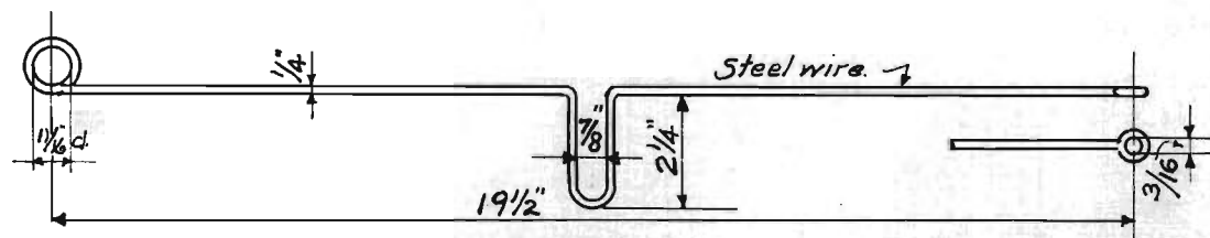
DETAIL OF WIRE SPRING. Scale: 3" = 1'-0"
