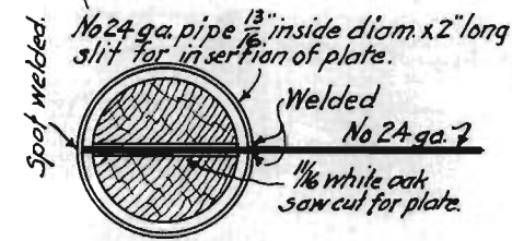
SECTION B-B. Full Size.
