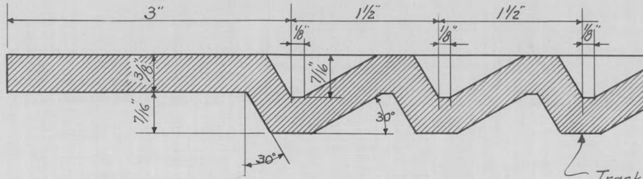
PART LONG. SECTION. Scale: Full Size.
