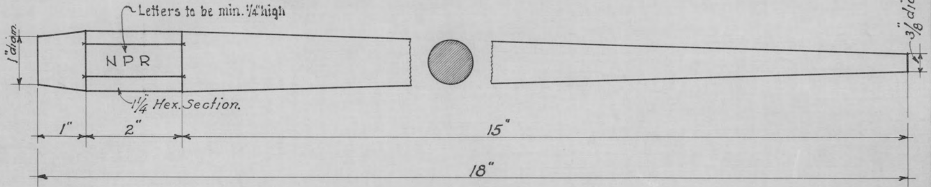
Side View.
