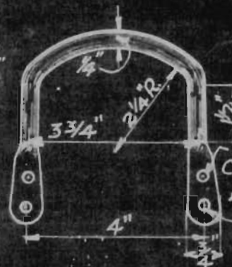
Detail of Handle. Scale: 4"=1'-0"
