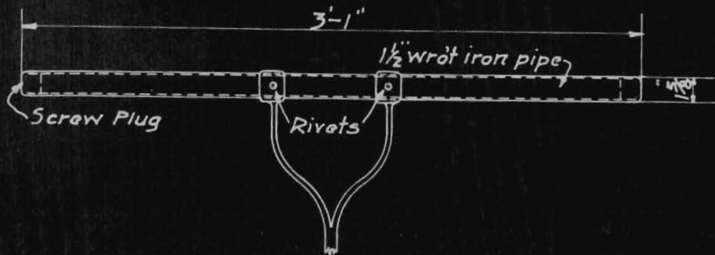
Detail of Metal Handle
