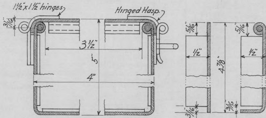
CROSS SECTION. PARTITION END SECTION. Scale: Full Size.
