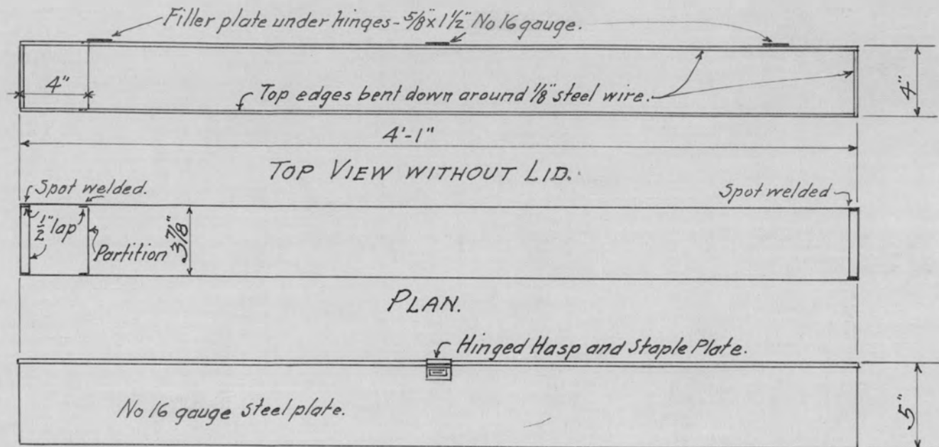
FRONT ELEVATION. Scale: 1\frac{1}{2} = 1'-0 "
