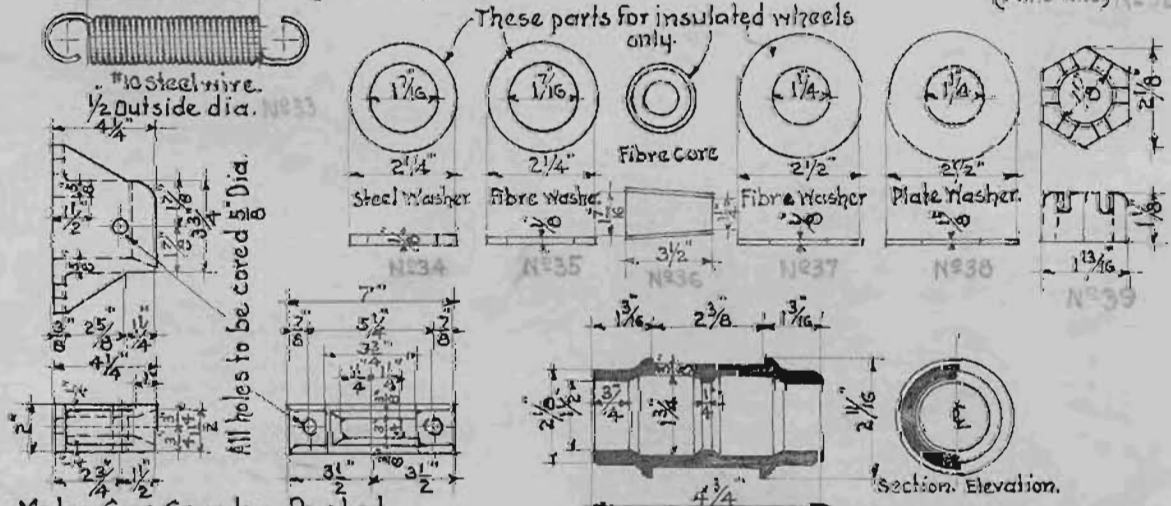
Motor Car Coupler Pocket. Mall. Iron Patt. H.M.-1 Scale-1 1/2"-1'-0"
